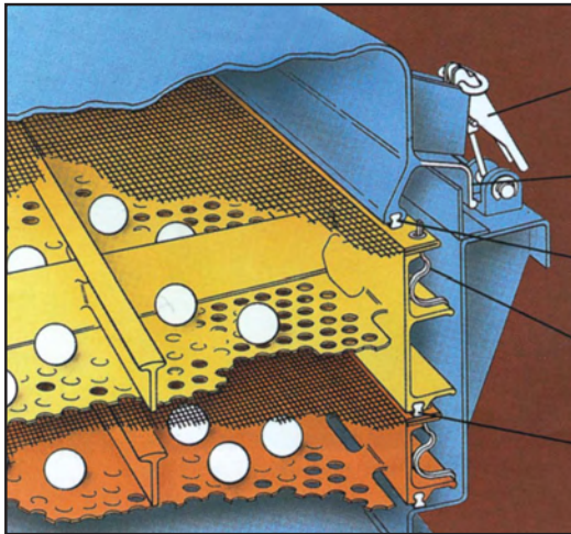
Aluminum Top Cover and Screen Frame Construction
