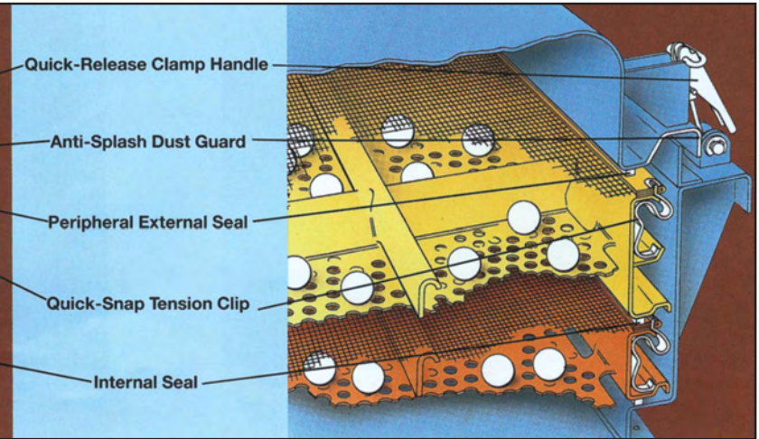
Steel Top Cover and Screen Frame Construction
